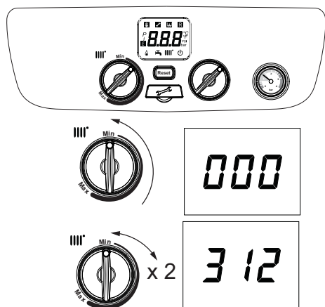
Fig.11 Enabling de-aeration function
